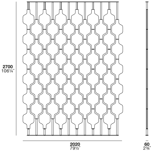
room divider ACC.200.12
